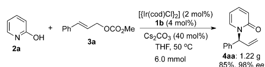
Scheme 3. A gram-scale synthesis of 4aa .
