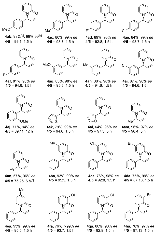
Scheme 2. Reaction substrate scope. Reaction conditions: 2 mol % of [\text{Ir}(\text{cod})\text{Cl}]_2 , 4 mol % of ( S,S,S )- 1b , 0.4 mmol of 3 , 0.8 mmol of 2 , and 0.16 mmol of \text{Cs}_2\text{CO}_3 in 4.0 mL THF at 50 °C. The ratio of 4/5 and N/O selectivity were determined by ^1\text{H} NMR analysis of the crude reaction mixture. Catalyst was prepared by n PrNH 2 activation. Unless noted, N/O > 95:5. [a] Yield of isolated 4 . [b] The ee value of 4 was determined by HPLC analysis. [c] N/O = 86:14.
