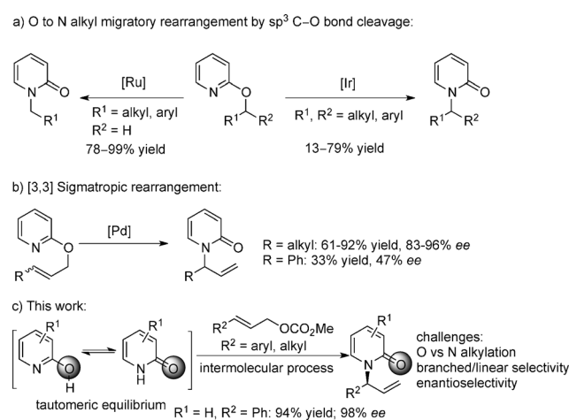
Scheme 1. Synthesis of N-substituted pyridones.
