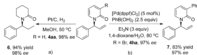
Scheme 4. Transformation of the products. dppf = 1,1'-bis(diphenylphosphino)ferrocene.
